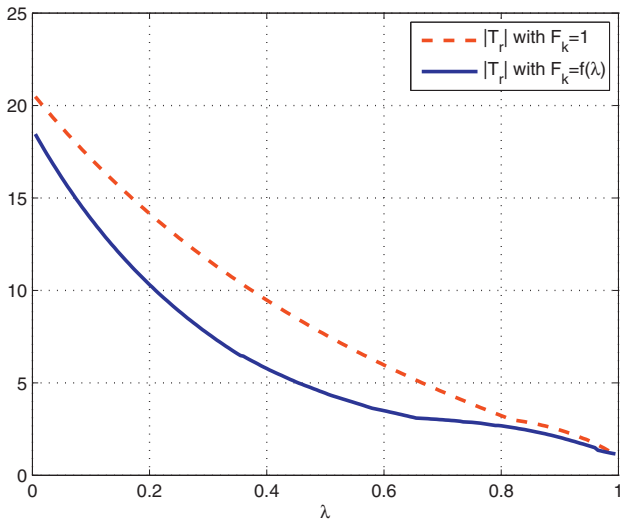
Fig. 5. Plot of T_r in (28) and (23) respectively.
