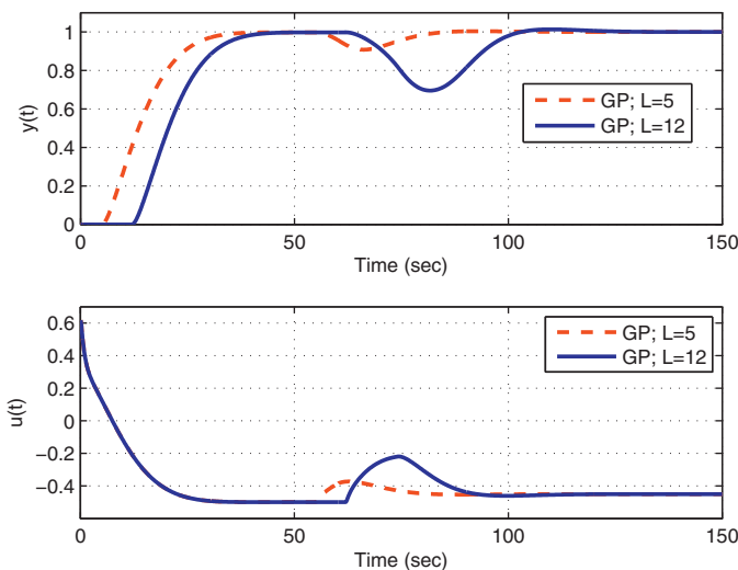
Fig. 24. Nominal system responses for a -0.05 step load disturbance at t=100s (Example 5).
