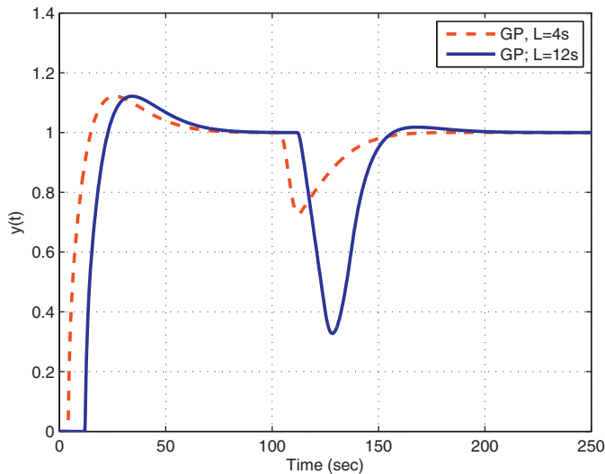
Fig. 13. Nominal system responses for a -0.05 step disturbance at t = 100s (Example 2).
