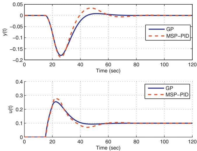
Fig. 19. Nominal system responses for a -0.1 step disturbance at t = 10s (Example 4).
