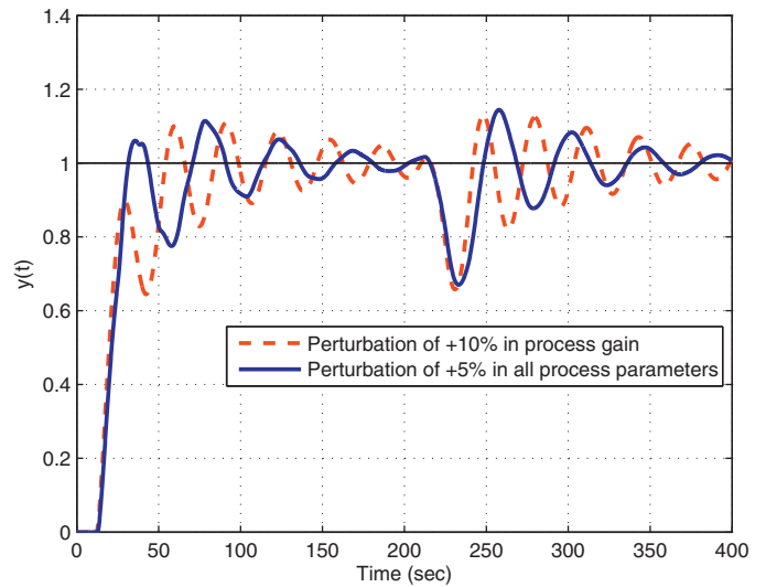
Fig. 25. Perturbed system responses for a -0.05 step load disturbance at t=200s (Example 5).
