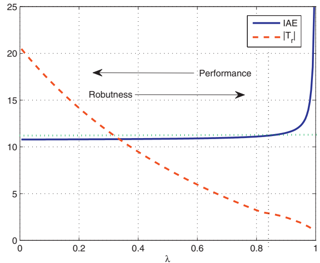
Fig. 4. Plot of IAE and T_r according to (26) and (28) respectively (Example 1).
