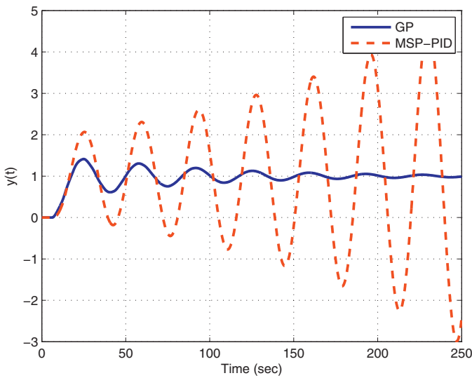
Fig. 23. Closed loop responses for the perturbed case when the time delay is increased by 25% and other parameters are decreased by -25% (Example 4)
