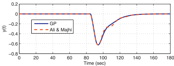
Fig. 9. Responses for a change of 20% in process gain (Example 1).
