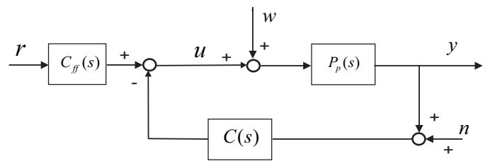
Fig. 18. MSP-PID control structure proposed in [19].
