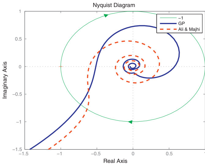
Fig. 8. Nyquist plots for Example 1.
