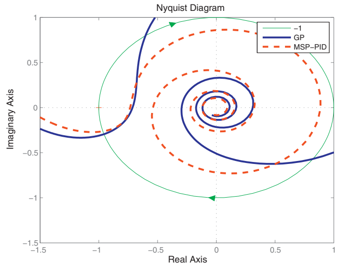
Fig. 21. Nyquist plots for Example 4.
