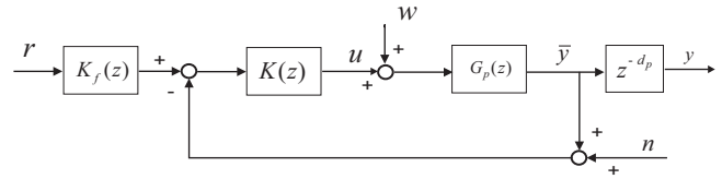
Fig. 1. Ideal delay-free loop.
