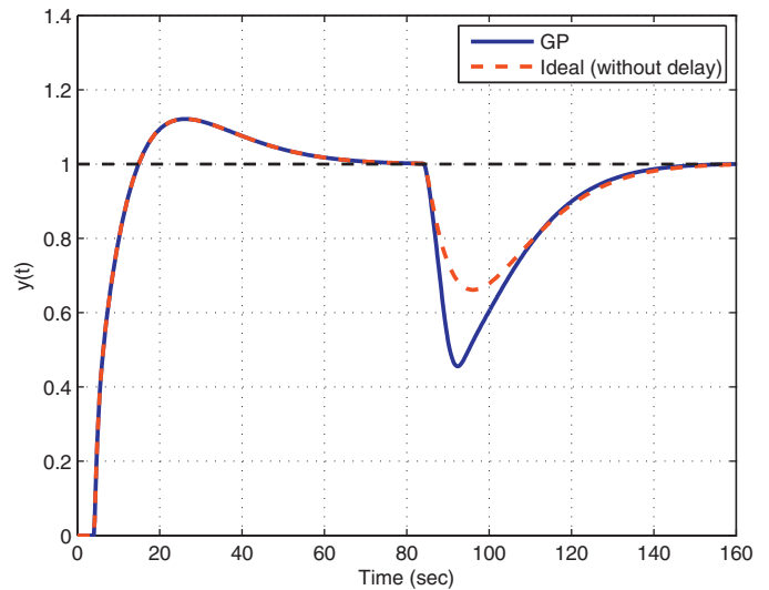
Fig. 6. Nominal output response compared with the ideal closed-loop system free of delay for a unit step change in the reference and a step load disturbance of -0.1 at t=80 s. (Example 1).
