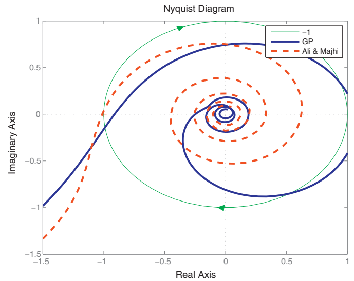
Fig. 11. Nyquist plots, for the perturbed case when time delay and gain are increased by 40% (Example 1).
