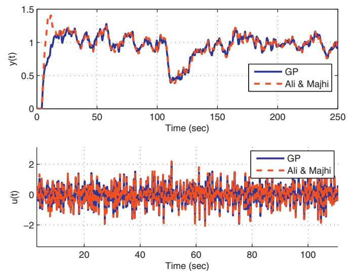
Fig. 12. Nominal system responses for white-noise measurement (Example 1).
