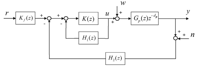
Fig. 3. Simplified control structure for analysis proposes.
