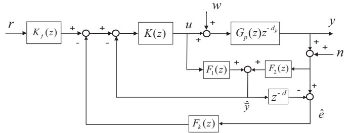
Fig. 2. Predictor-based control structure.
