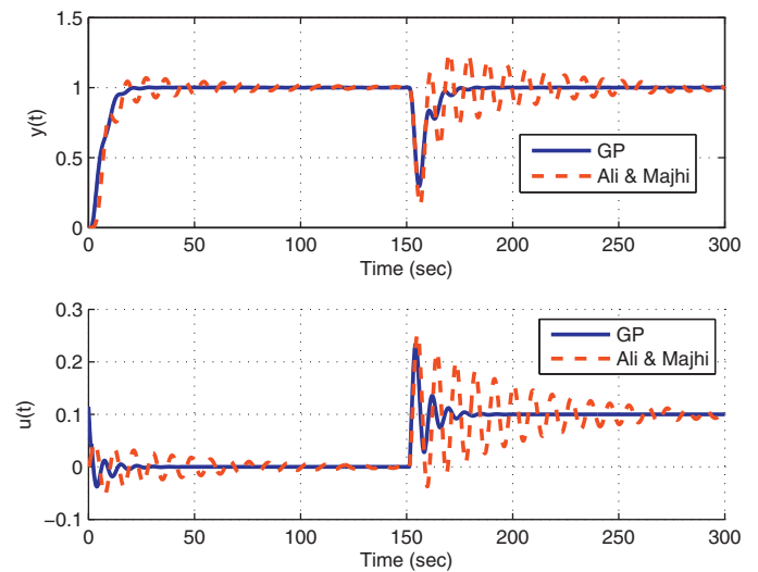
Fig. 17. Closed loop responses for the perturbed case when the delay and gain are increased by 25% (Example 3).
