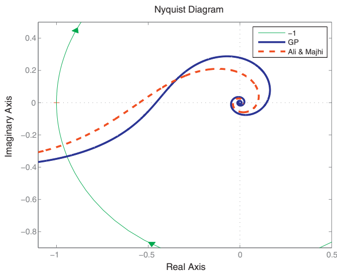
Fig. 16. Nyquist plots for Example 3.
