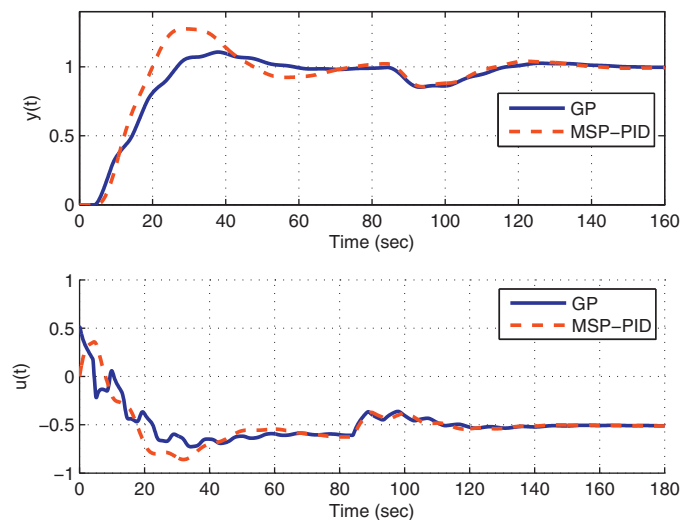
Fig. 22. Perturbed system responses; all process parameters are changed by -18\% (Example 4).
