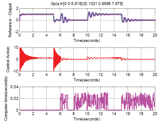
Figure 6: Switching control due to interferences.
