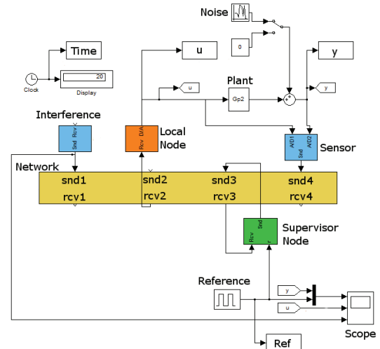
Figure 4: Control kernel implementation and simulation.
